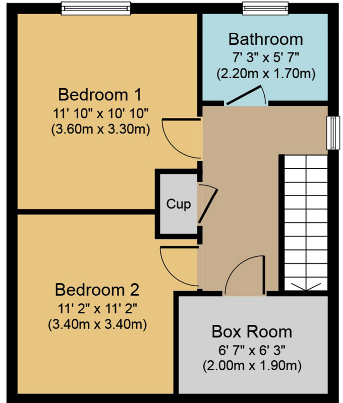
First Floor Approximate Floor Area 429 sq. ft. (39.9 sq. m.)
